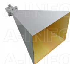
LB-284-20-C-7/16F Standard Gain Horn Antenna 2.6-3.95GHz 20dB Gain 7/16(DIN) Female
